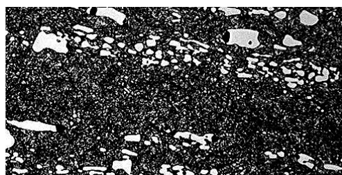
Microstructure Tool Steel AISI D2, 12% Cr
